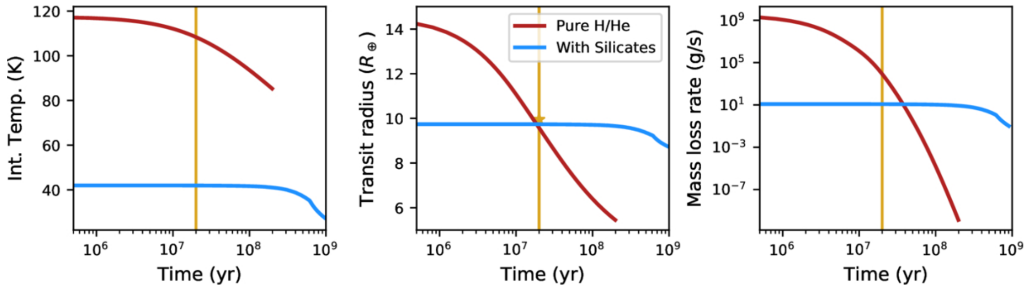
Figure 8. from Saugata Barat et al 2025 Astron. J. 170 doi:10.3847/1538-3881/ade89 https://dx.doi.org/10.3847/1538-3881/ade89 © 2025. The Author(s). Published by the American Astronomical Society.
