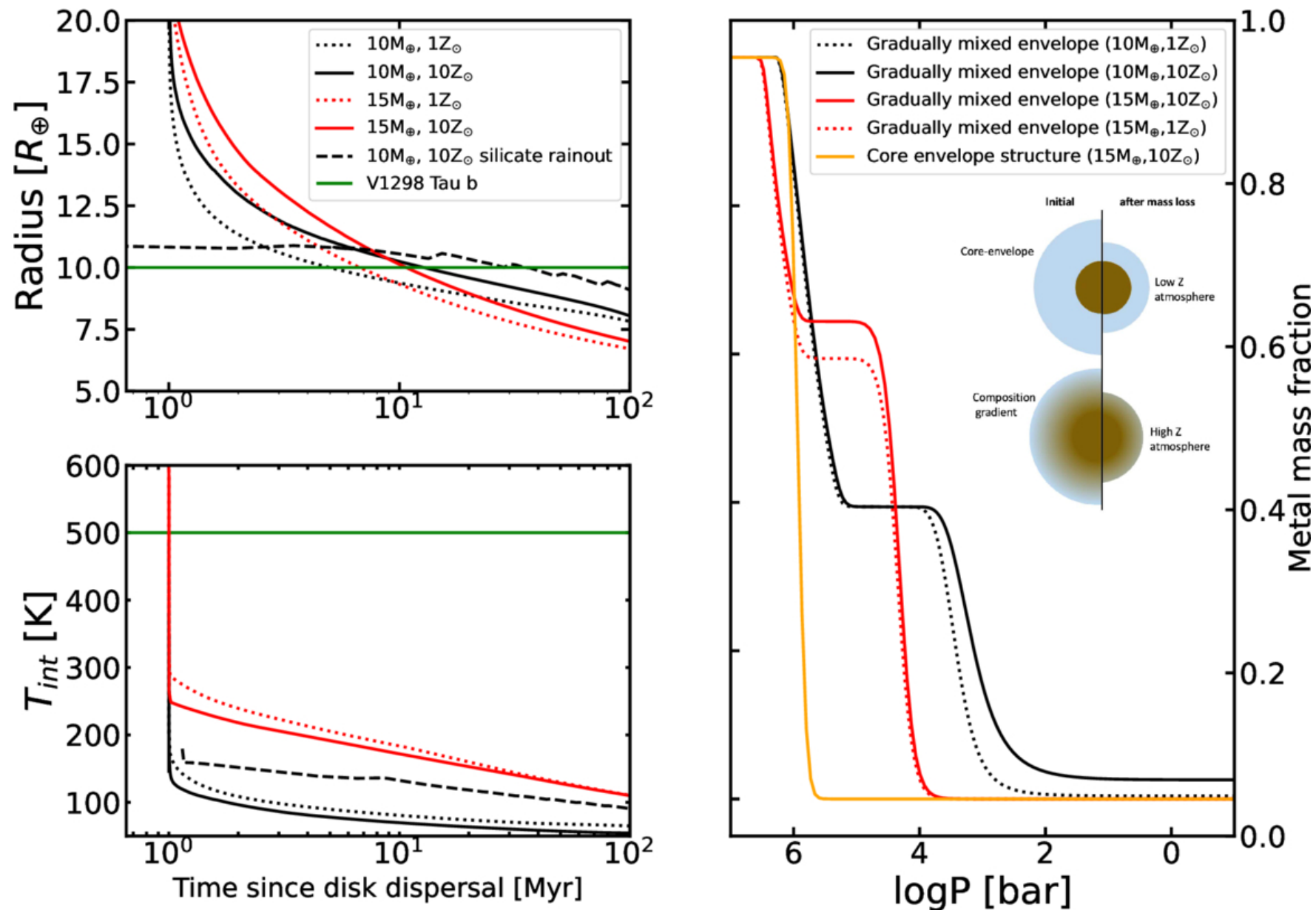
Figure 7. from Saugata Barat et al 2025 Astron. J. 170 doi:10.3847/1538-3881/ade89 https://dx.doi.org/10.3847/1538-3881/ade89 © 2025. The Author(s). Published by the American Astronomical Society.
