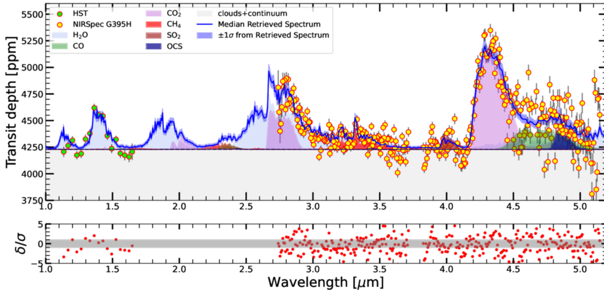
Figure 3. from Saugata Barat et al 2025 Astron. J. 170 doi:10.3847/1538-3881/ade89 https://dx.doi.org/10.3847/1538-3881/ade89 © 2025. The Author(s). Published by the American Astronomical Society.
