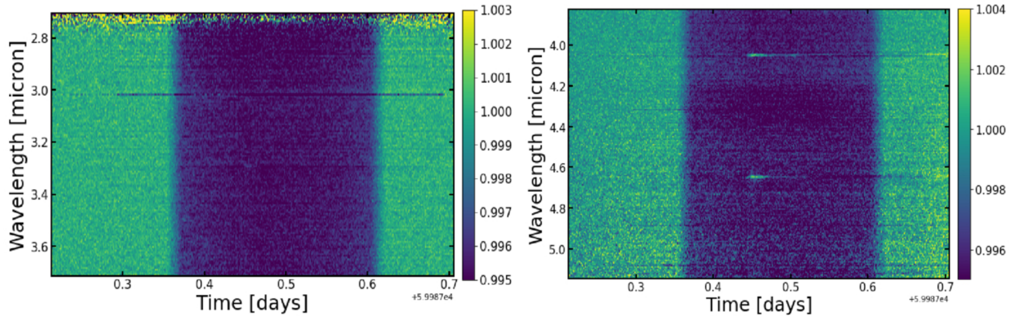
Figure 2. from Saugata Barat et al 2025 Astron. J. 170 doi:10.3847/1538-3881/ade89 https://dx.doi.org/10.3847/1538-3881/ade89 © 2025. The Author(s). Published by the American Astronomical Society.
