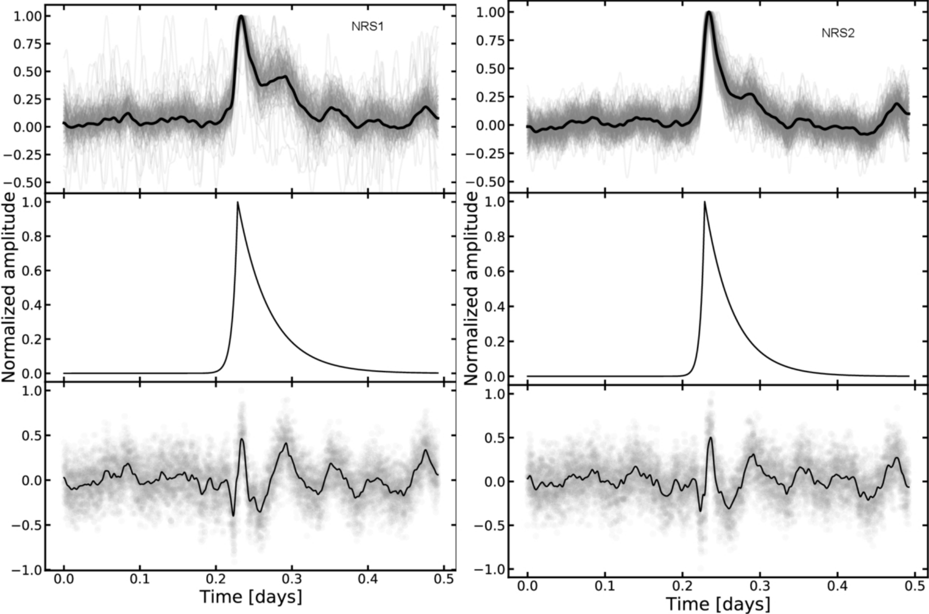
Figure C3. from Saugata Barat et al 2025 Astron. J. 170 doi:10.3847/1538-3881/ade89 https://dx.doi.org/10.3847/1538-3881/ade89 © 2025. The Author(s). Published by the American Astronomical Society.
