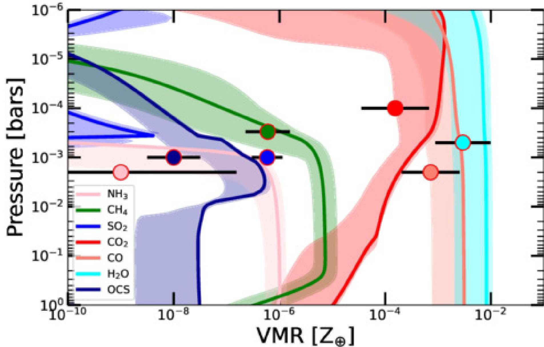
Figure 10. from Saugata Barat et al 2025 Astron. J. 170 doi:10.3847/1538-3881/ade89 https://dx.doi.org/10.3847/1538-3881/ade89 © 2025. The Author(s). Published by the American Astronomical Society.
