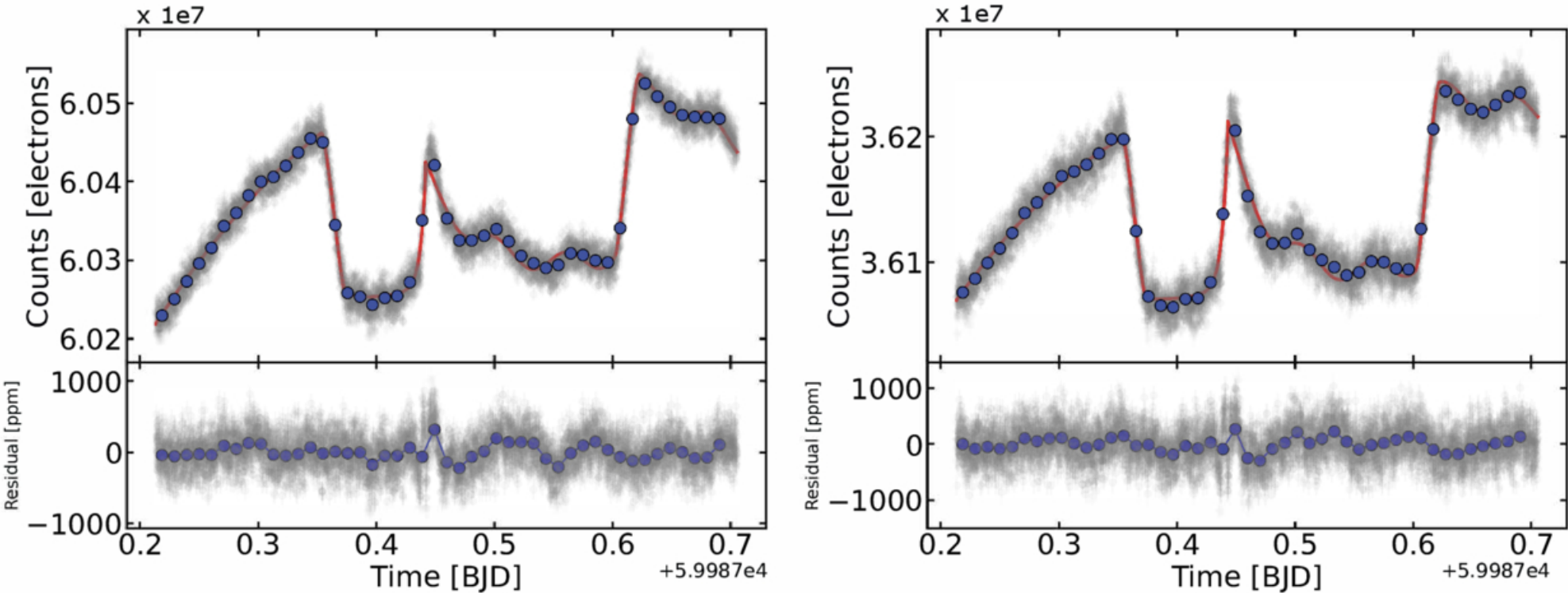
Figure 1. from Saugata Barat et al 2025 Astron. J. 170 doi:10.3847/1538-3881/ade89 https://dx.doi.org/10.3847/1538-3881/ade89 © 2025. The Author(s). Published by the American Astronomical Society.
