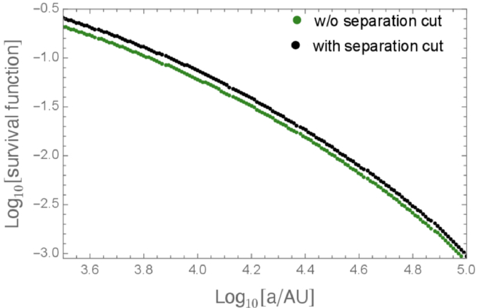
Figure 6. from Valeri V. Makarov 2025 Astron. J. 170 doi:10.3847/1538-3881/ade79 https://dx.doi.org/10.3847/1538-3881/ade79 © 2025. The Author(s). Published by the American Astronomical Society.
