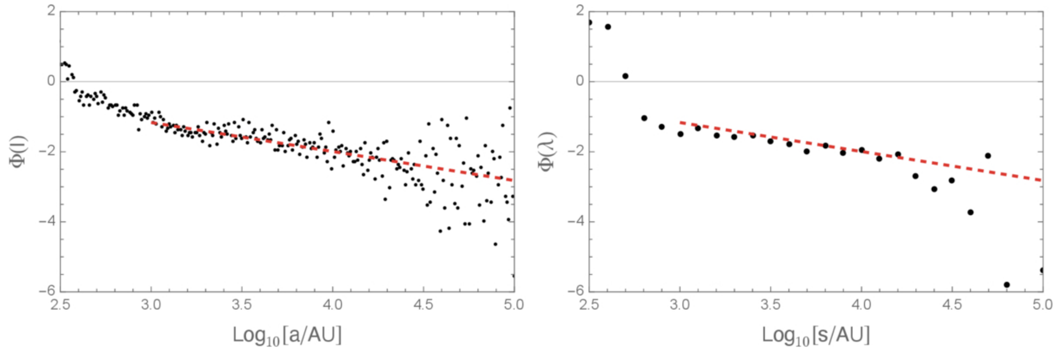
Figure 3. from Valeri V. Makarov 2025 Astron. J. 170 doi:10.3847/1538-3881/ade79 https://dx.doi.org/10.3847/1538-3881/ade79 © 2025. The Author(s). Published by the American Astronomical Society.
