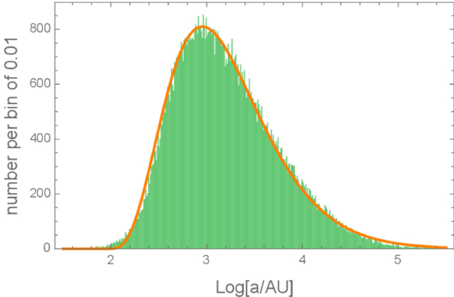
Figure 2. from Valeri V. Makarov 2025 Astron. J. 170 doi:10.3847/1538-3881/ade79 https://dx.doi.org/10.3847/1538-3881/ade79 © 2025. The Author(s). Published by the American Astronomical Society.
