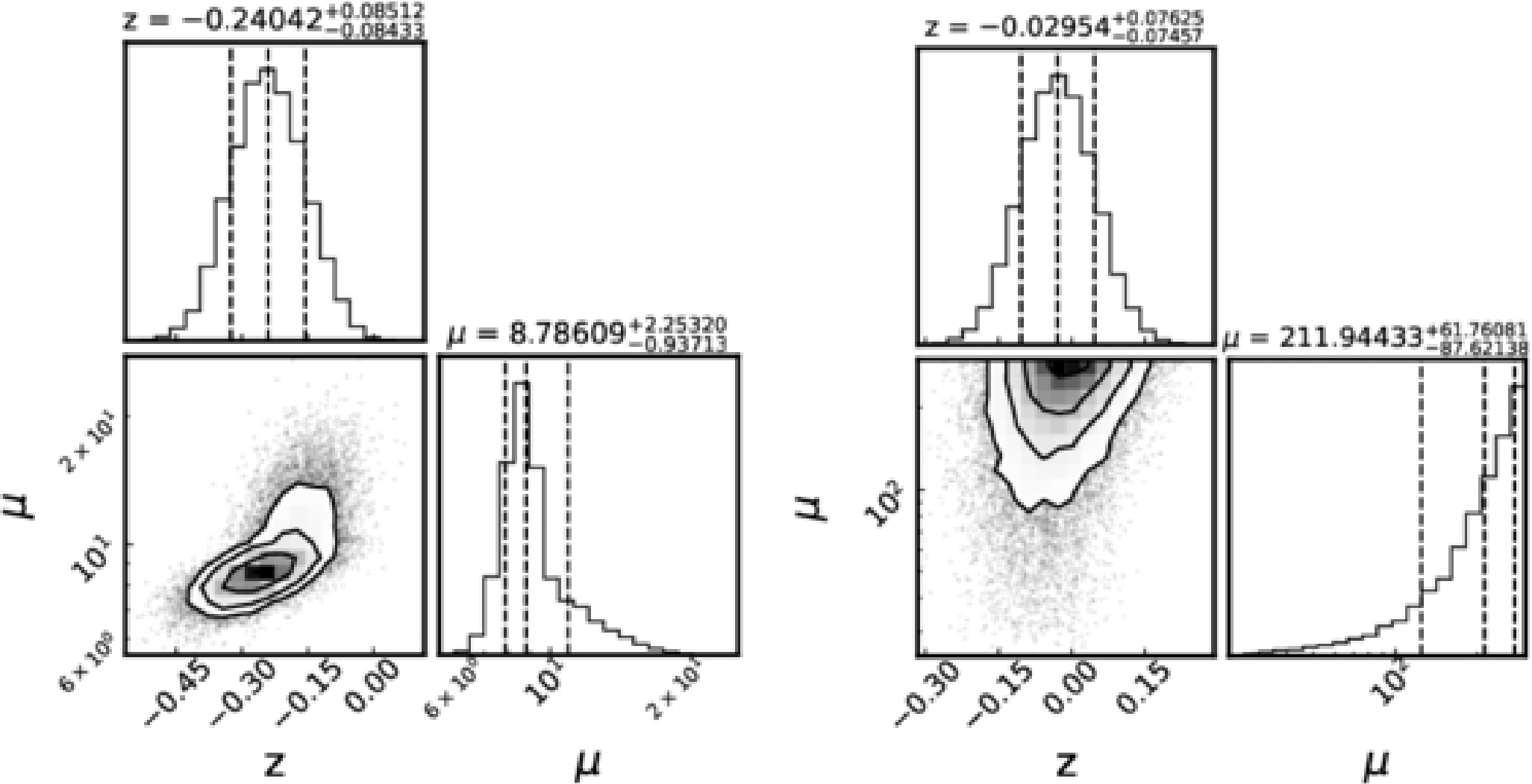
Figure A1. from Déreck-Alexandre Lizotte et al 2025 Astron. J. 170 doi:10.3847/1538-3881/adeb82 https://dx.doi.org/10.3847/1538-3881/adeb82 © 2025. The Author(s). Published by the American Astronomical Society.
