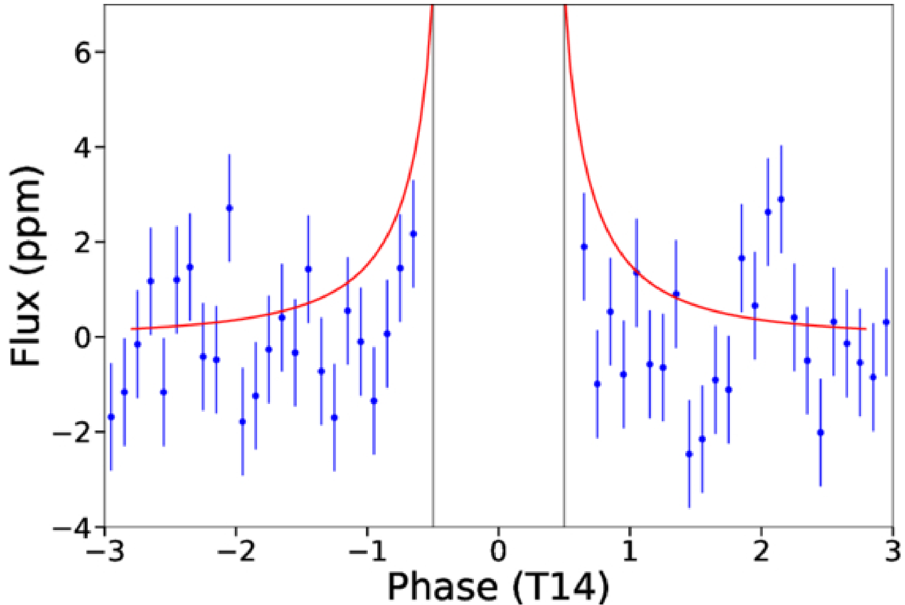
Figure 5. from Déreck-Alexandre Lizotte et al 2025 Astron. J. 170 doi:10.3847/1538-3881/adeb82 https://dx.doi.org/10.3847/1538-3881/adeb82 © 2025. The Author(s). Published by the American Astronomical Society.
