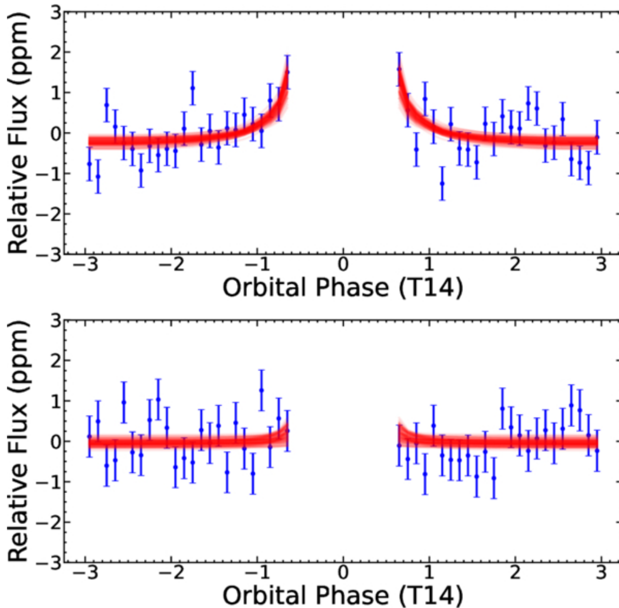
Figure 2. from Déreck-Alexandre Lizotte et al 2025 Astron. J. 170 doi:10.3847/1538-3881/adeb82 https://dx.doi.org/10.3847/1538-3881/adeb82 © 2025. The Author(s). Published by the American Astronomical Society.
