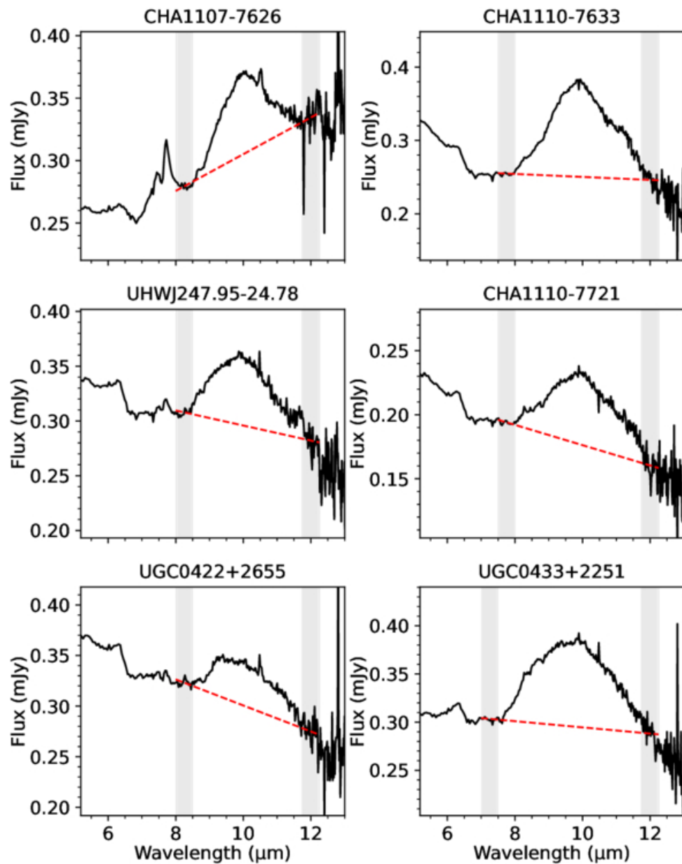
Figure 8. from Belinda Damian et al 2025 Astron. J. 170 doi:10.3847/1538-3881/adea50 https://dx.doi.org/10.3847/1538-3881/adea50 © 2025. The Author(s). Published by the American Astronomical Society.
