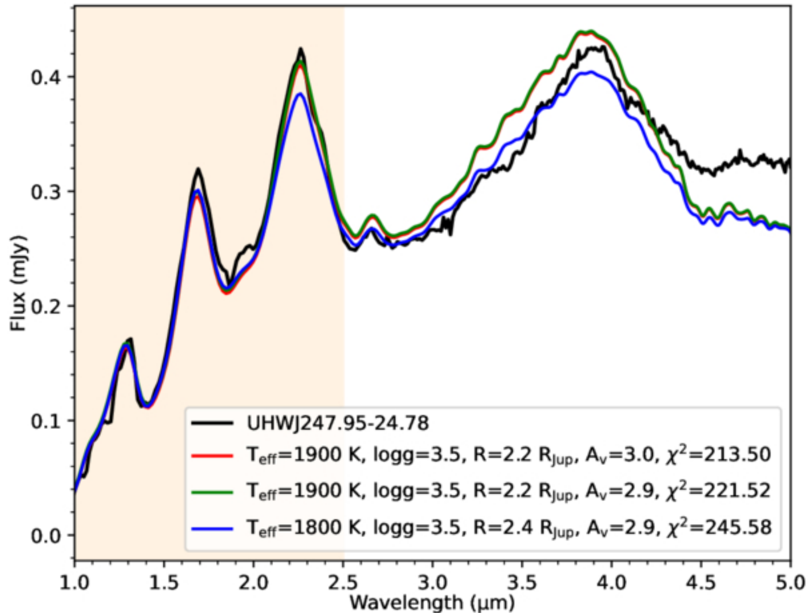
Figure 4. from Belinda Damian et al 2025 Astron. J. 170 doi:10.3847/1538-3881/adea50 https://dx.doi.org/10.3847/1538-3881/adea50 © 2025. The Author(s). Published by the American Astronomical Society.
