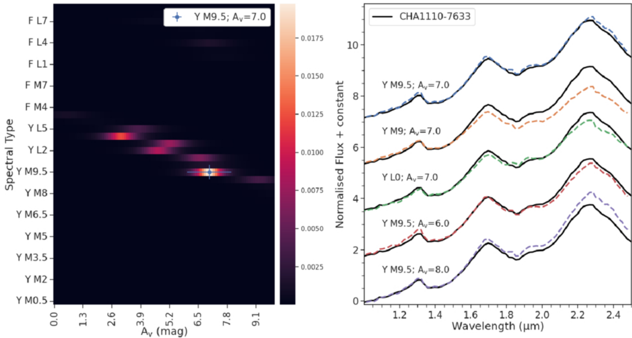
Figure 3. from Belinda Damian et al 2025 Astron. J. 170 doi:10.3847/1538-3881/adea50 https://dx.doi.org/10.3847/1538-3881/adea50 © 2025. The Author(s). Published by the American Astronomical Society.
