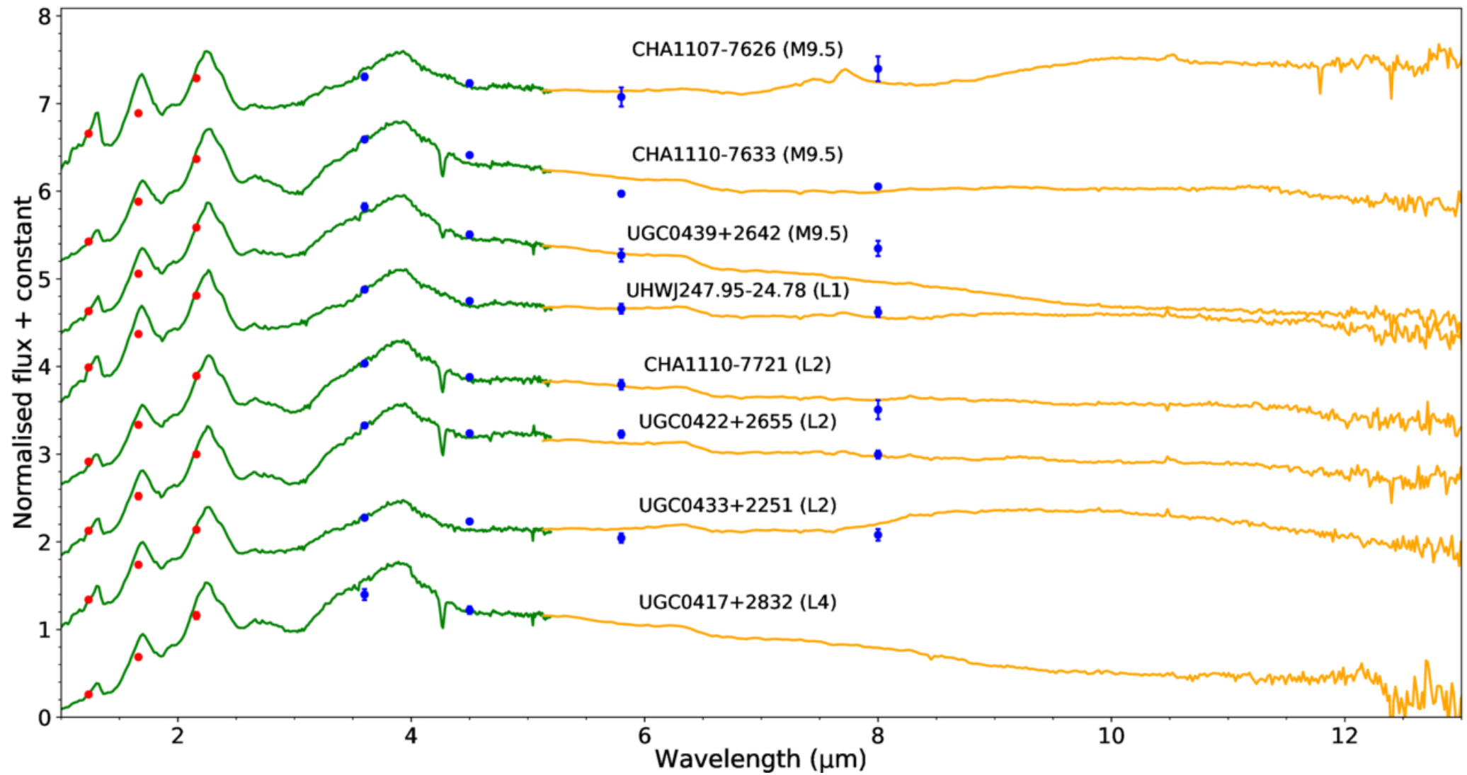
Figure 2. from Belinda Damian et al 2025 Astron. J. 170 doi:10.3847/1538-3881/adea50 https://dx.doi.org/10.3847/1538-3881/adea50 © 2025. The Author(s). Published by the American Astronomical Society.
