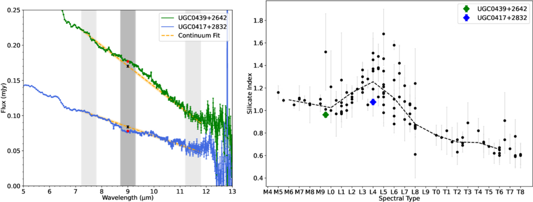
Figure 11. from Belinda Damian et al 2025 Astron. J. 170 doi:10.3847/1538-3881/adea50 https://dx.doi.org/10.3847/1538-3881/adea50 © 2025. The Author(s). Published by the American Astronomical Society.
