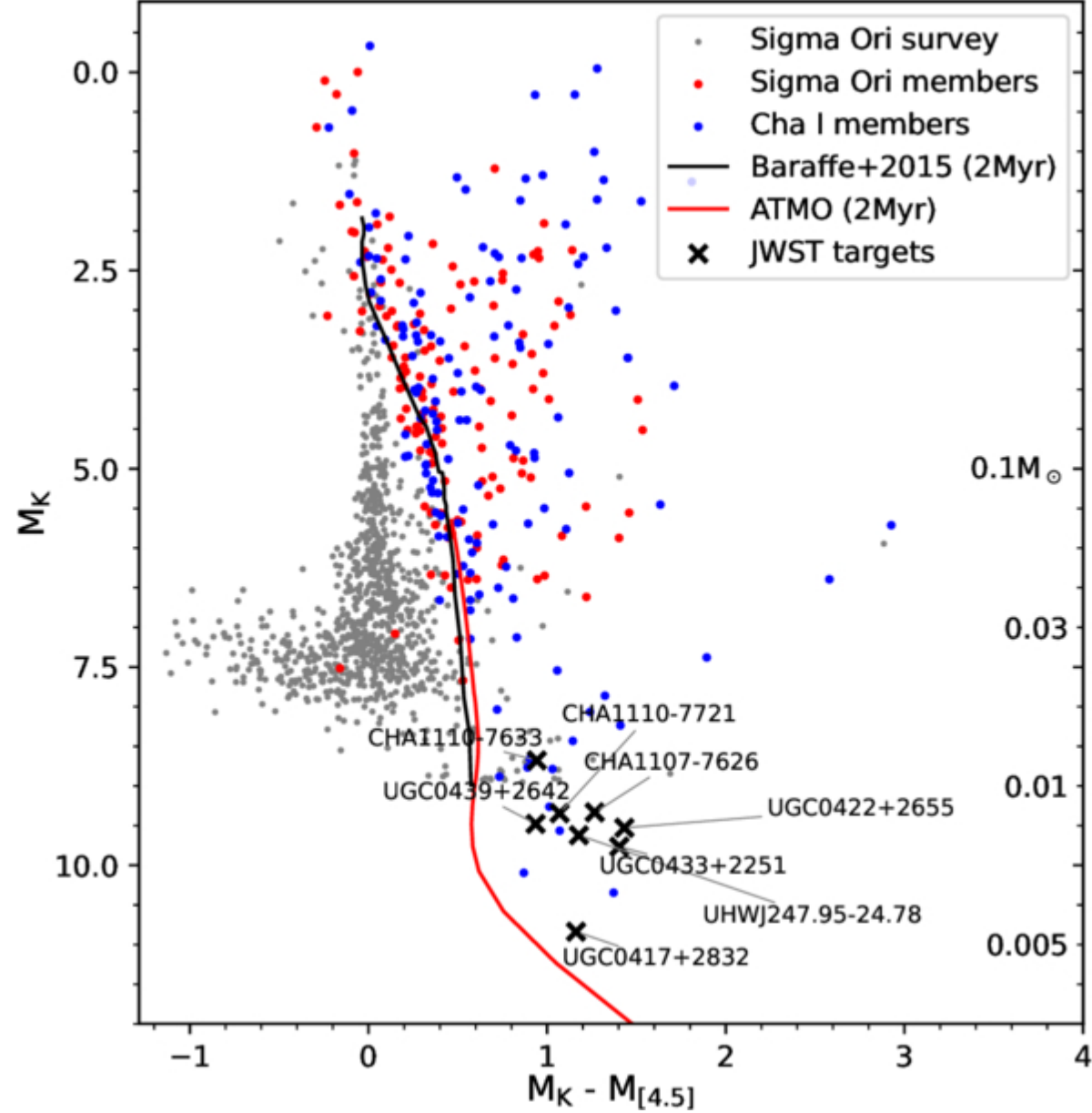
Figure 1. from Belinda Damian et al 2025 Astron. J. 170 doi:10.3847/1538-3881/adea50 https://dx.doi.org/10.3847/1538-3881/adea50 © 2025. The Author(s). Published by the American Astronomical Society.
