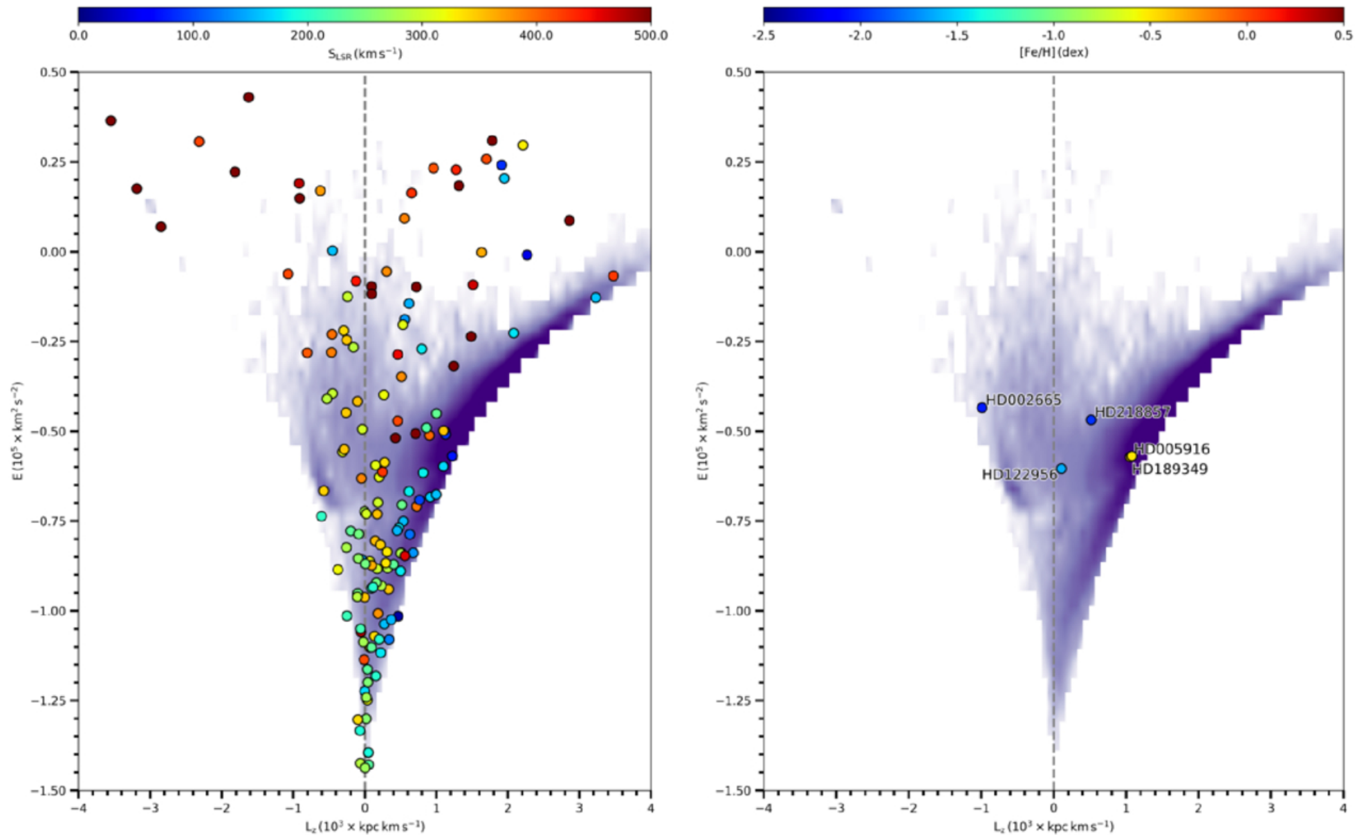
Figure 8. from Gizay Yolalan et al 2025 Astron. J. 170 doi:10.3847/1538-3881/ade9aa https://dx.doi.org/10.3847/1538-3881/ade9aa © 2025. The Author(s). Published by the American Astronomical Society.
