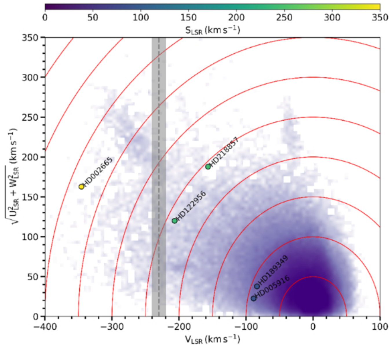
Figure 5. from Gizay Yolalan et al 2025 Astron. J. 170 doi:10.3847/1538-3881/ade9aa https://dx.doi.org/10.3847/1538-3881/ade9aa © 2025. The Author(s). Published by the American Astronomical Society.
