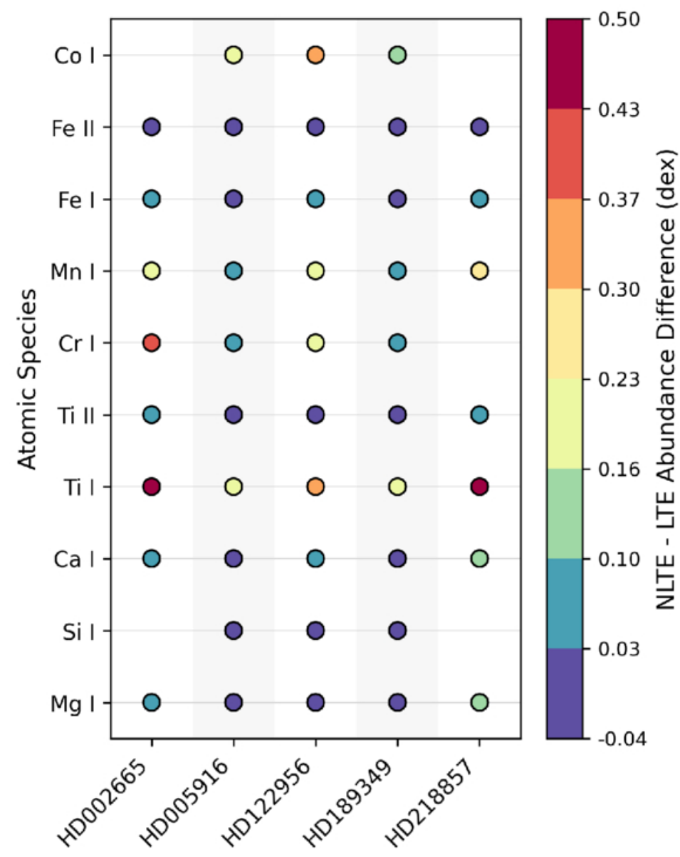
Figure 3. from Gizay Yolalan et al 2025 Astron. J. 170 doi:10.3847/1538-3881/ade9aa https://dx.doi.org/10.3847/1538-3881/ade9aa © 2025. The Author(s). Published by the American Astronomical Society.
