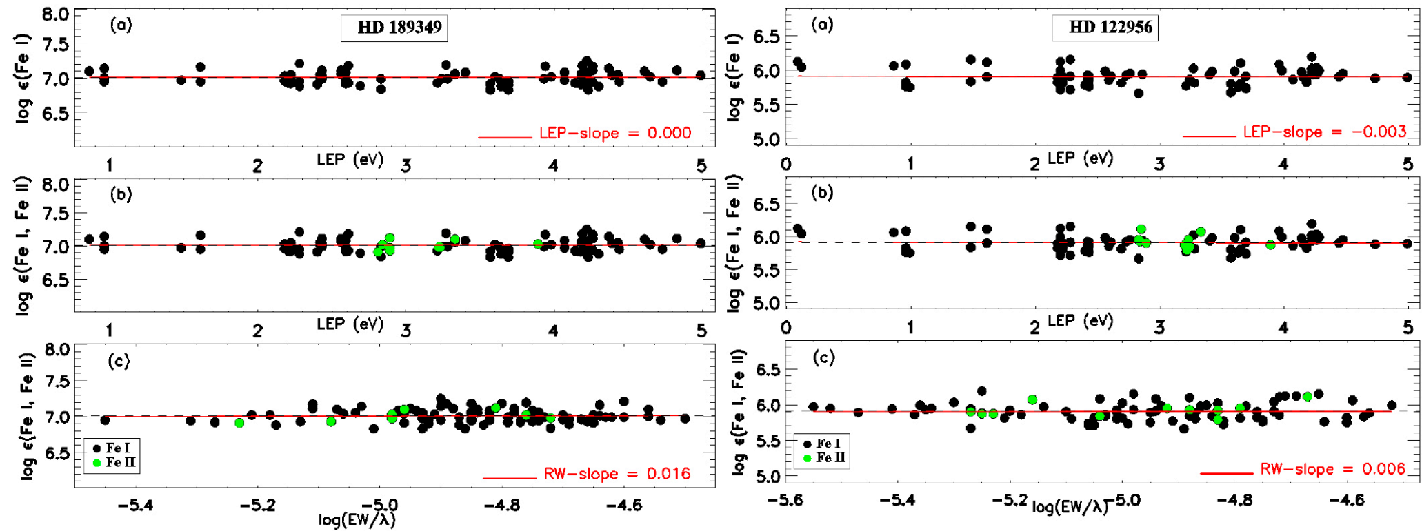
Figure 2. from Gizay Yolalan et al 2025 Astron. J. 170 doi:10.3847/1538-3881/ade9aa https://dx.doi.org/10.3847/1538-3881/ade9aa © 2025. The Author(s). Published by the American Astronomical Society.
