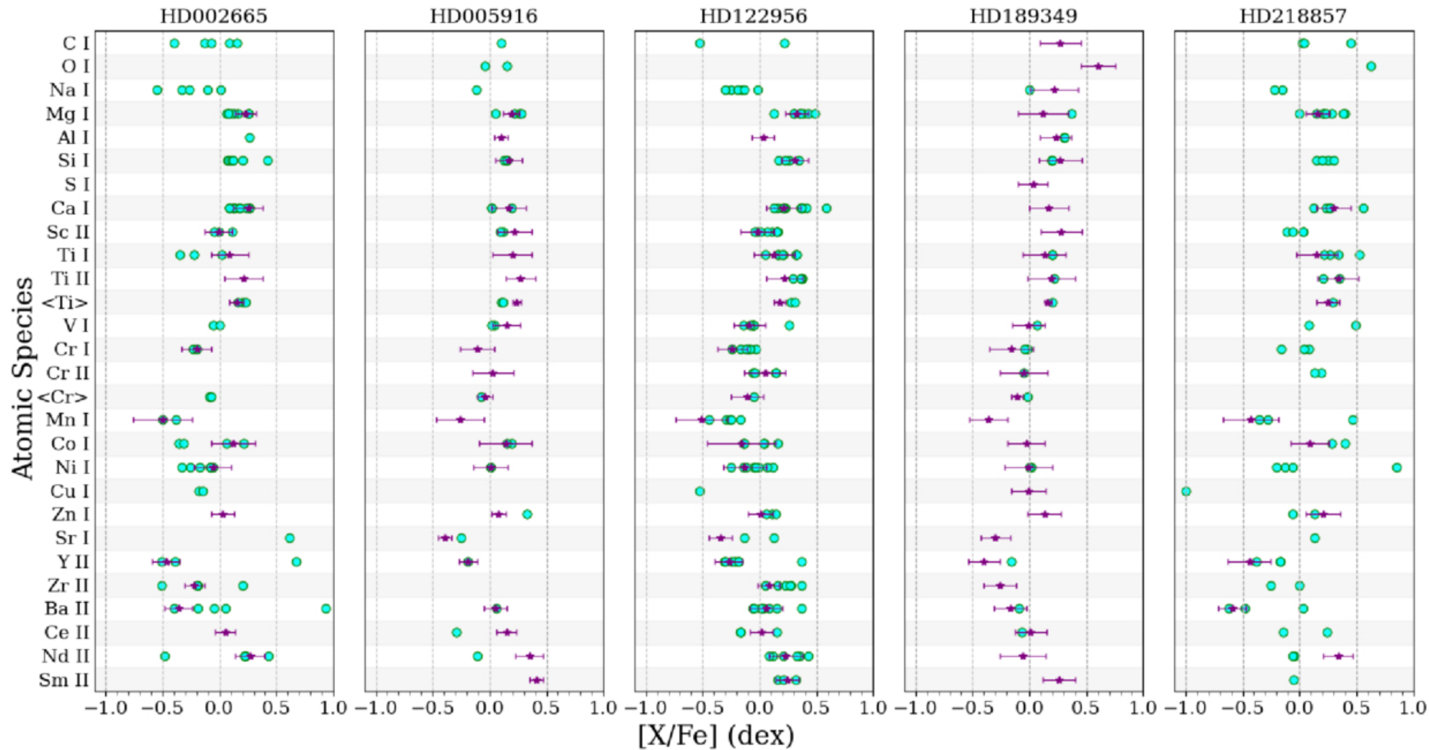
Figure 10. from Gizay Yolalan et al 2025 Astron. J. 170 doi:10.3847/1538-3881/ade9aa https://dx.doi.org/10.3847/1538-3881/ade9aa © 2025. The Author(s). Published by the American Astronomical Society.
