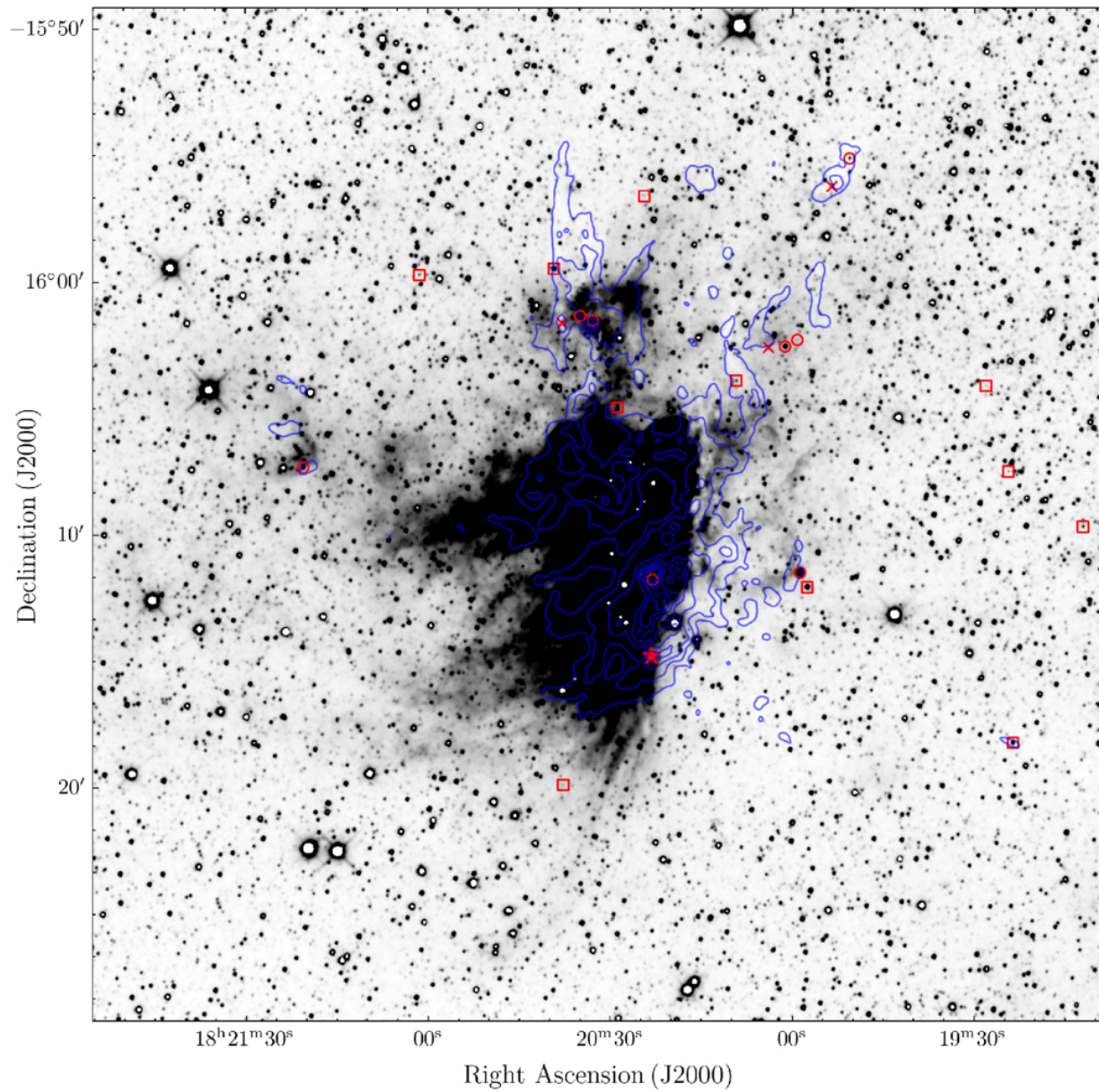
Figure 9. from Zhiwei Chen et al 2025 Astron. J. 170 doi:10.3847/1538-3881/ade988 https://dx.doi.org/10.3847/1538-3881/ade988 © 2025. The Author(s). Published by the American Astronomical Society.
