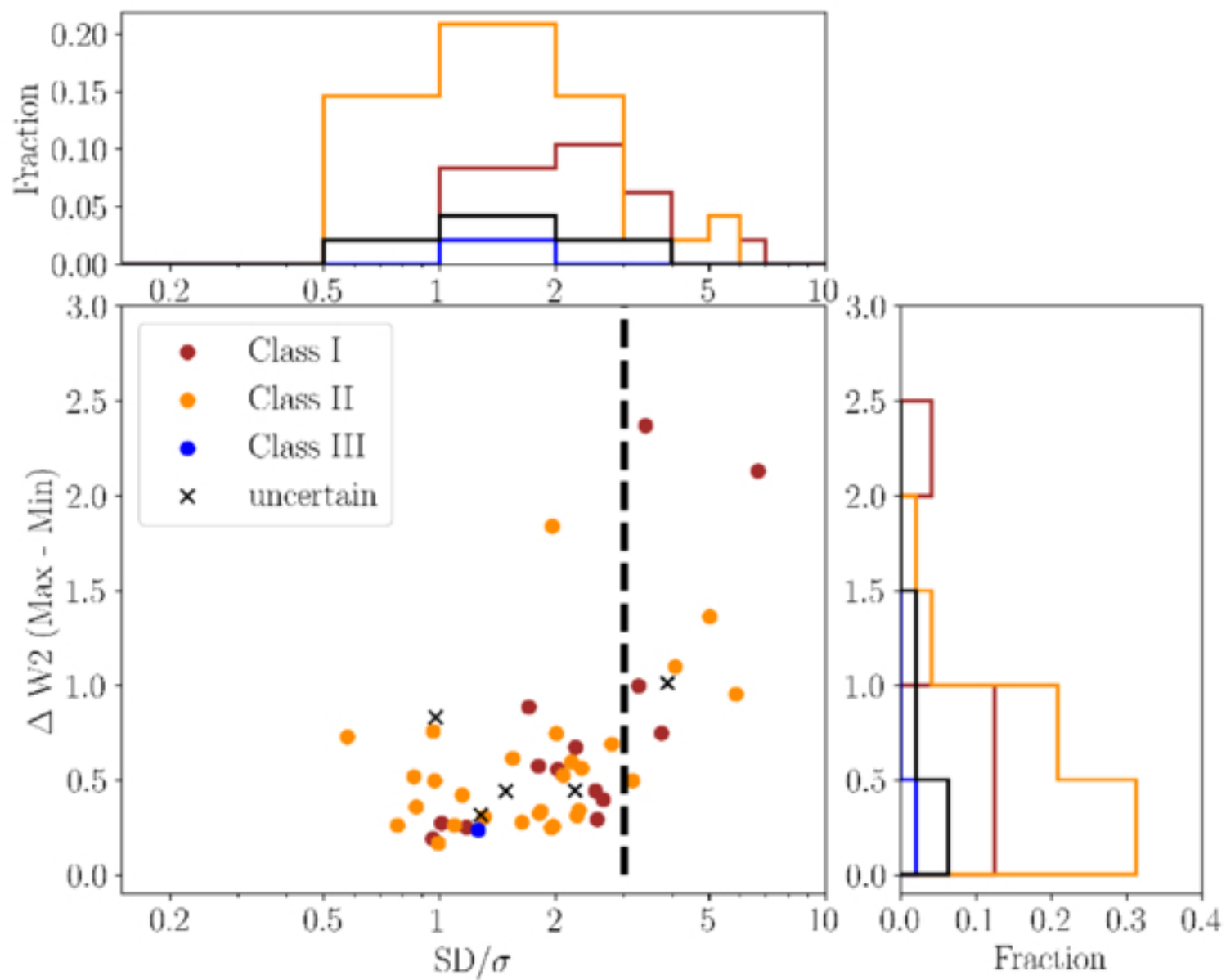
Figure 6. from Zhiwei Chen et al 2025 Astron. J. 170 doi:10.3847/1538-3881/ade988 https://dx.doi.org/10.3847/1538-3881/ade988 © 2025. The Author(s). Published by the American Astronomical Society.
