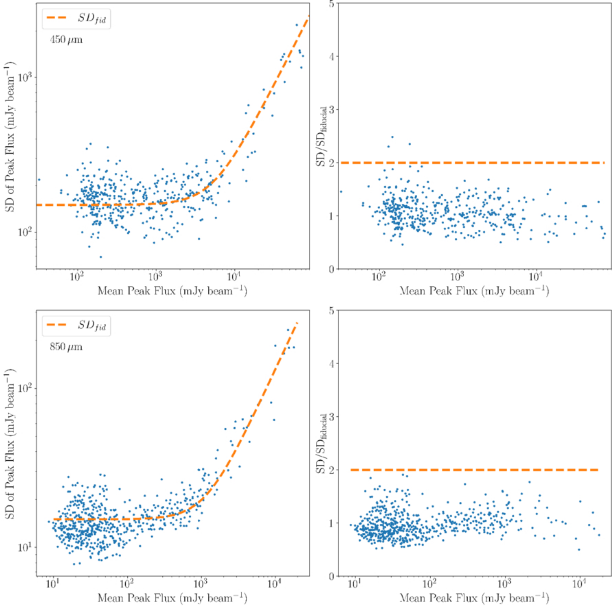
Figure 3. from Zhiwei Chen et al 2025 Astron. J. 170 doi:10.3847/1538-3881/ade988 https://dx.doi.org/10.3847/1538-3881/ade988 © 2025. The Author(s). Published by the American Astronomical Society.
