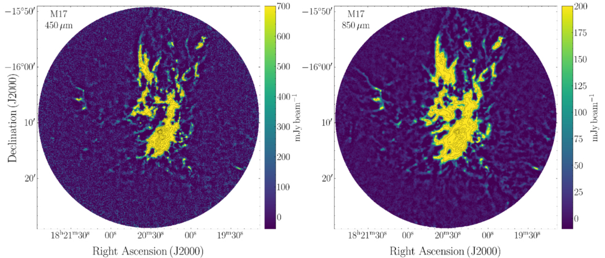
Figure 2. from Zhiwei Chen et al 2025 Astron. J. 170 doi:10.3847/1538-3881/ade988 https://dx.doi.org/10.3847/1538-3881/ade988 © 2025. The Author(s). Published by the American Astronomical Society.
