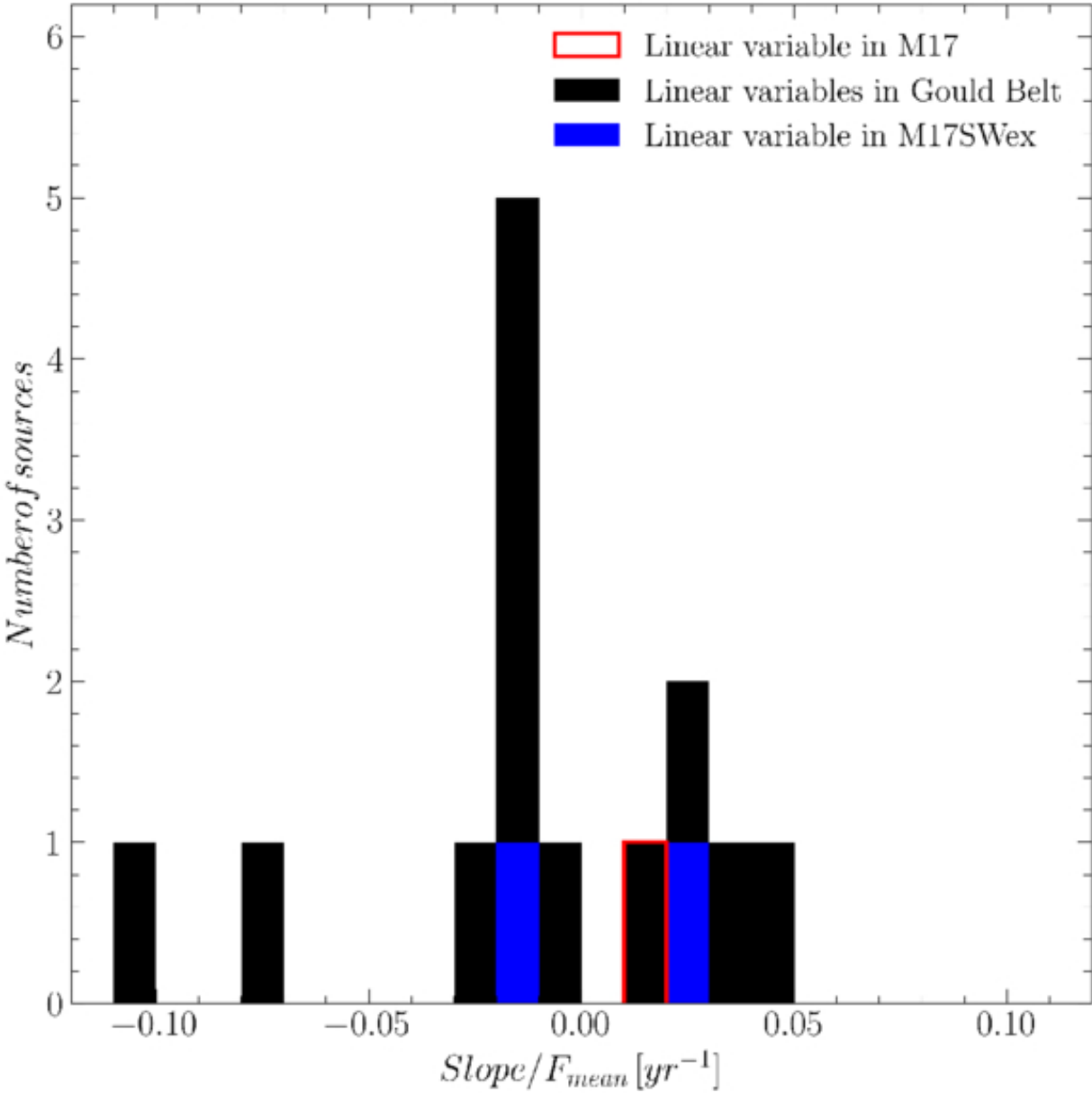
Figure 15. from Zhiwei Chen et al 2025 Astron. J. 170 doi:10.3847/1538-3881/ade988 https://dx.doi.org/10.3847/1538-3881/ade988 © 2025. The Author(s). Published by the American Astronomical Society.
