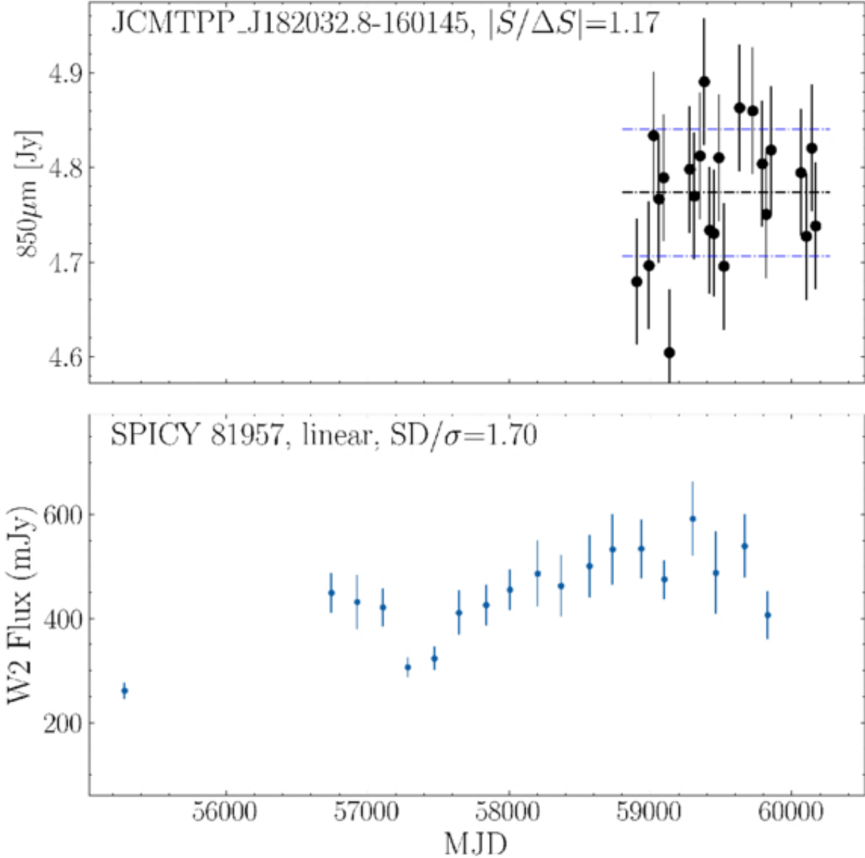
Figure 10. from Zhiwei Chen et al 2025 Astron. J. 170 doi:10.3847/1538-3881/ade988 https://dx.doi.org/10.3847/1538-3881/ade988 © 2025. The Author(s). Published by the American Astronomical Society.
