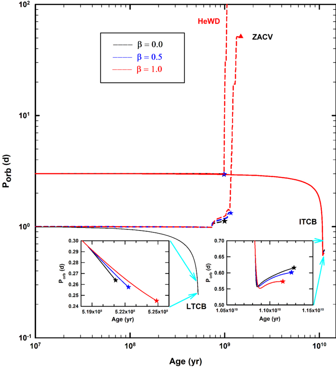
Figure 8. from Somayeh Soomandar et al 2025 Astron. J. 170 doi:10.3847/1538-3881/ade985 https://dx.doi.org/10.3847/1538-3881/ade985 © 2025. The Author(s). Published by the American Astronomical Society.
