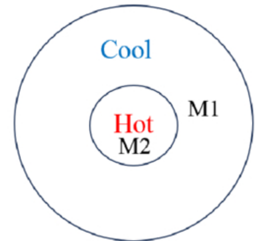
Secondary Eclipse
