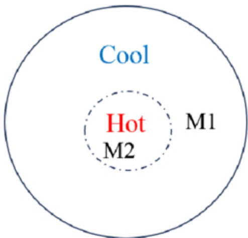
Primary Eclipse
