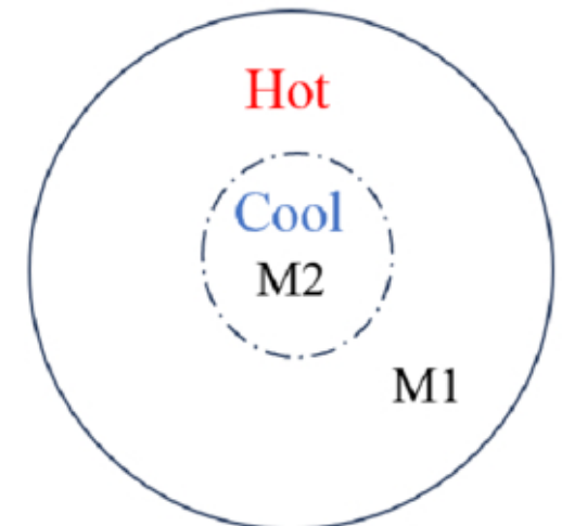
Secondary Eclipse
