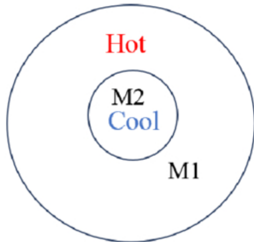
Primary Eclipse
