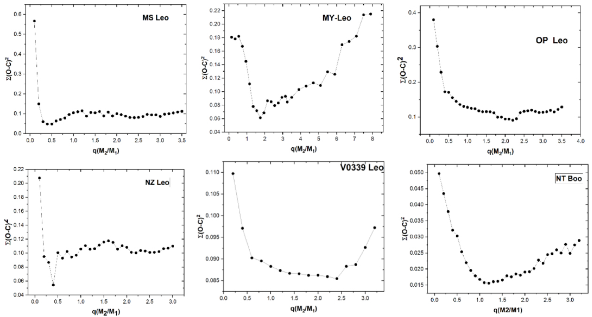
Figure 3. from Somayeh Soomandar et al 2025 Astron. J. 170 doi:10.3847/1538-3881/ade985 https://dx.doi.org/10.3847/1538-3881/ade985 © 2025. The Author(s). Published by the American Astronomical Society.
