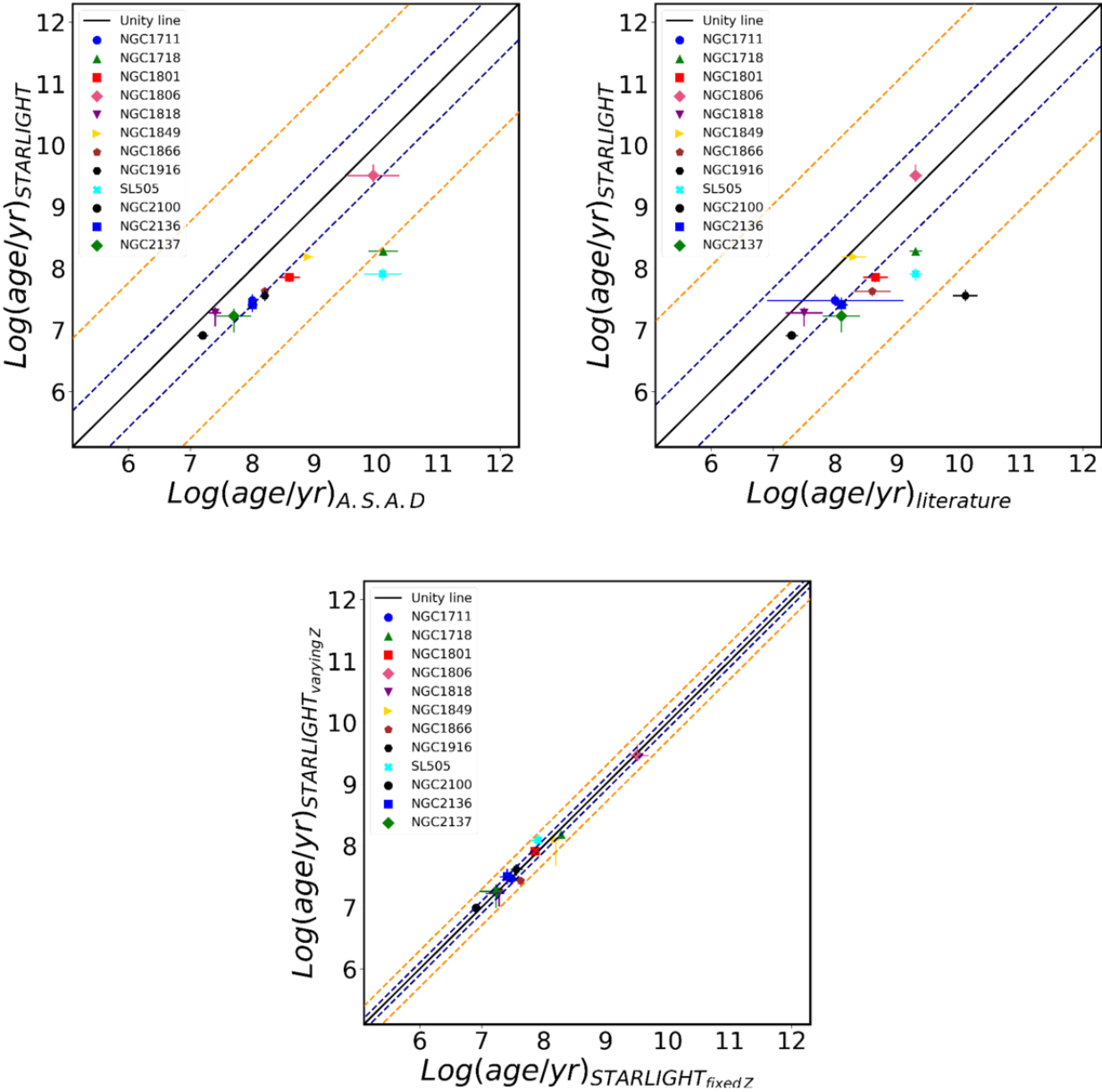
Figure 9. from Martina I. Tapia-Reina et al 2025 Astron. J. 170 doi:10.3847/1538-3881/ade703 https://dx.doi.org/10.3847/1538-3881/ade703 © 2025. The Author(s). Published by the American Astronomical Society.
