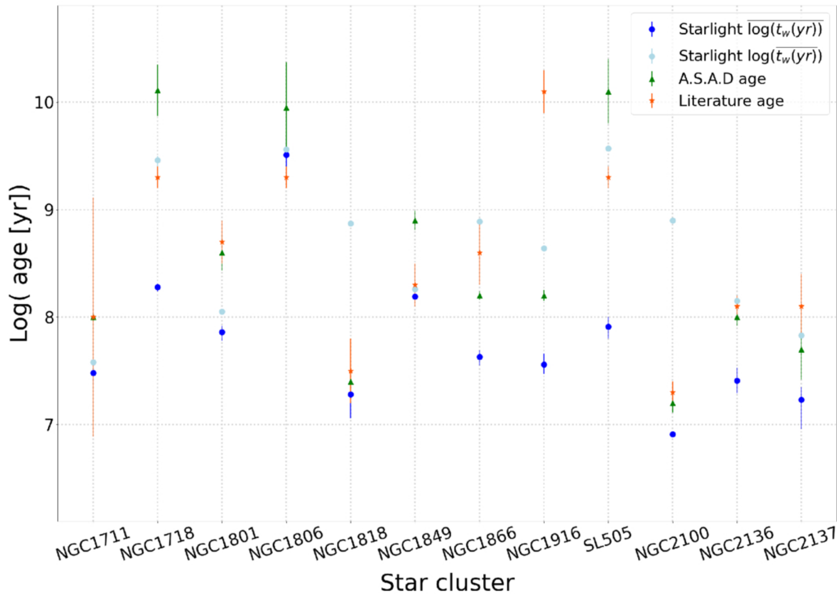
Figure 6. from Martina I. Tapia-Reina et al 2025 Astron. J. 170 doi:10.3847/1538-3881/ade703 https://dx.doi.org/10.3847/1538-3881/ade703 © 2025. The Author(s). Published by the American Astronomical Society.
