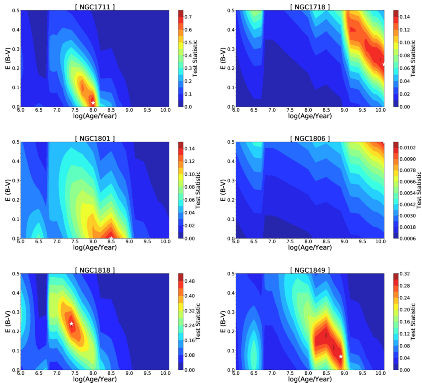
Figure 4. from Martina I. Tapia-Reina et al 2025 Astron. J. 170 doi:10.3847/1538-3881/ade703 https://dx.doi.org/10.3847/1538-3881/ade703 © 2025. The Author(s). Published by the American Astronomical Society.
