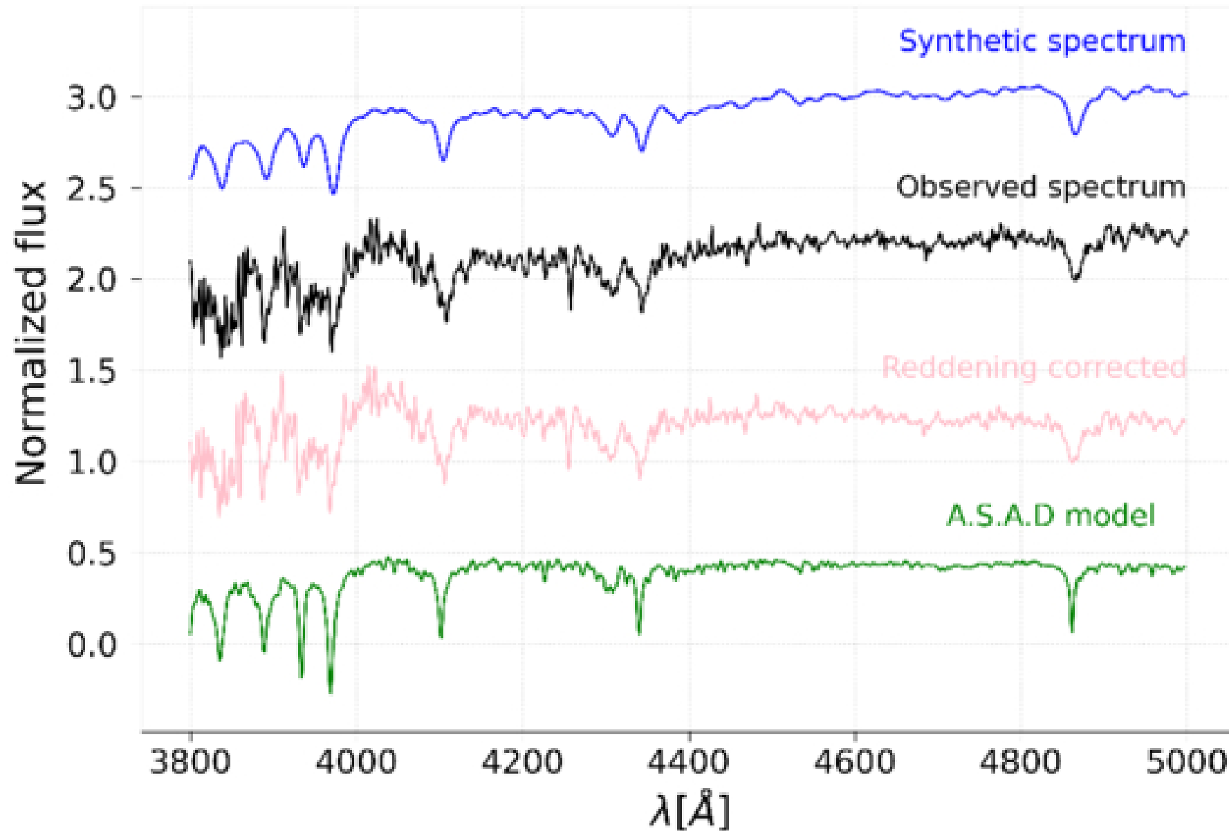
Figure 3. from Martina I. Tapia-Reina et al 2025 Astron. J. 170 doi:10.3847/1538-3881/ade703 https://dx.doi.org/10.3847/1538-3881/ade703 © 2025. The Author(s). Published by the American Astronomical Society.
