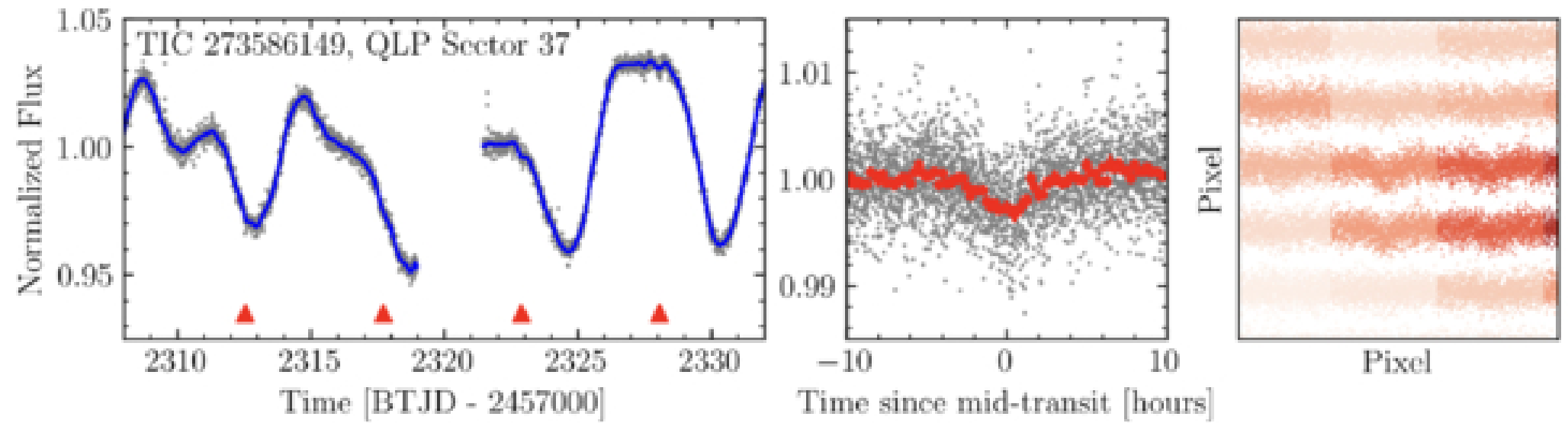
Figure 9. from Sydney Vach et al 2025 Astron. J. 170 doi:10.3847/1538-3881/ade67f https://dx.doi.org/10.3847/1538-3881/ade67f © 2025. The Author(s). Published by the American Astronomical Society.
