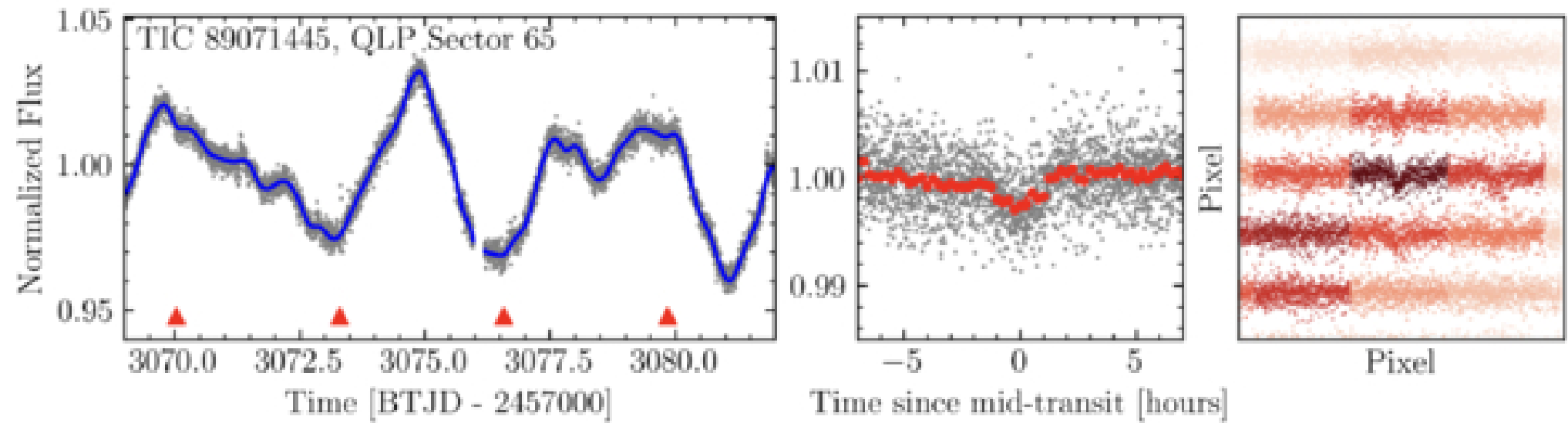
Figure 8. from Sydney Vach et al 2025 Astron. J. 170 doi:10.3847/1538-3881/ade67f https://dx.doi.org/10.3847/1538-3881/ade67f © 2025. The Author(s). Published by the American Astronomical Society.
