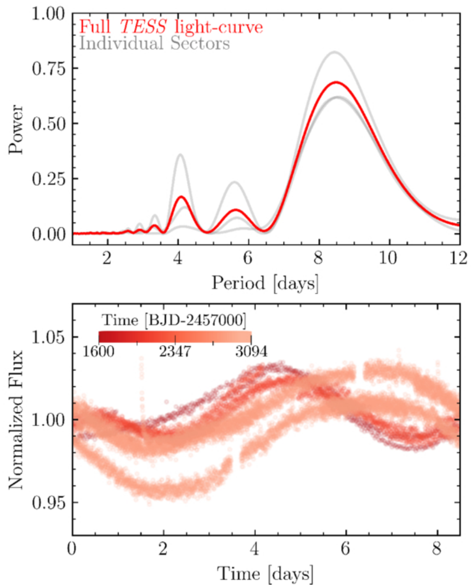
Figure 6. from Sydney Vach et al 2025 Astron. J. 170 doi:10.3847/1538-3881/ade67f https://dx.doi.org/10.3847/1538-3881/ade67f © 2025. The Author(s). Published by the American Astronomical Society.
