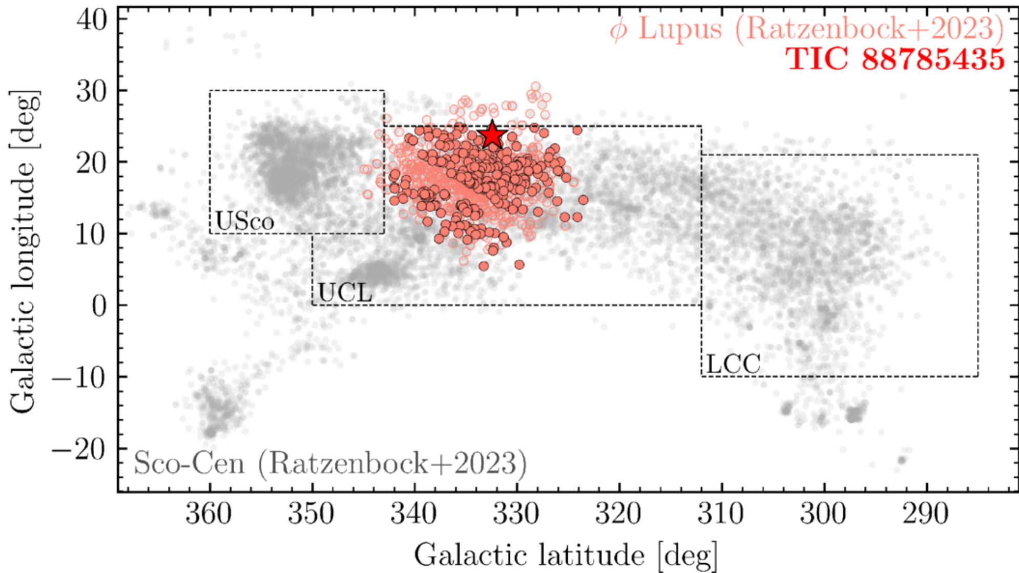
Figure 4. from Sydney Vach et al 2025 Astron. J. 170 doi:10.3847/1538-3881/ade67f https://dx.doi.org/10.3847/1538-3881/ade67f © 2025. The Author(s). Published by the American Astronomical Society.
