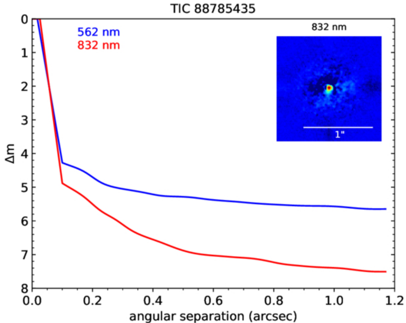
Figure 3. from Sydney Vach et al 2025 Astron. J. 170 doi:10.3847/1538-3881/ade67f https://dx.doi.org/10.3847/1538-3881/ade67f © 2025. The Author(s). Published by the American Astronomical Society.
