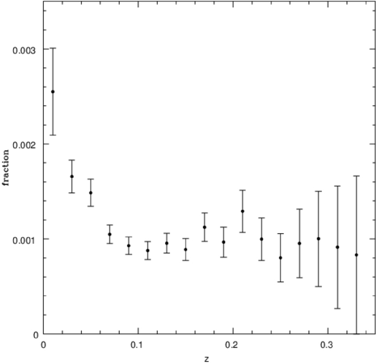
Figure 6. from Masafumi Yagi et al 2025 Astron. J. 170 doi:10.3847/1538-3881/ade543 https://dx.doi.org/10.3847/1538-3881/ade543 © 2025. The Author(s). Published by the American Astronomical Society.
