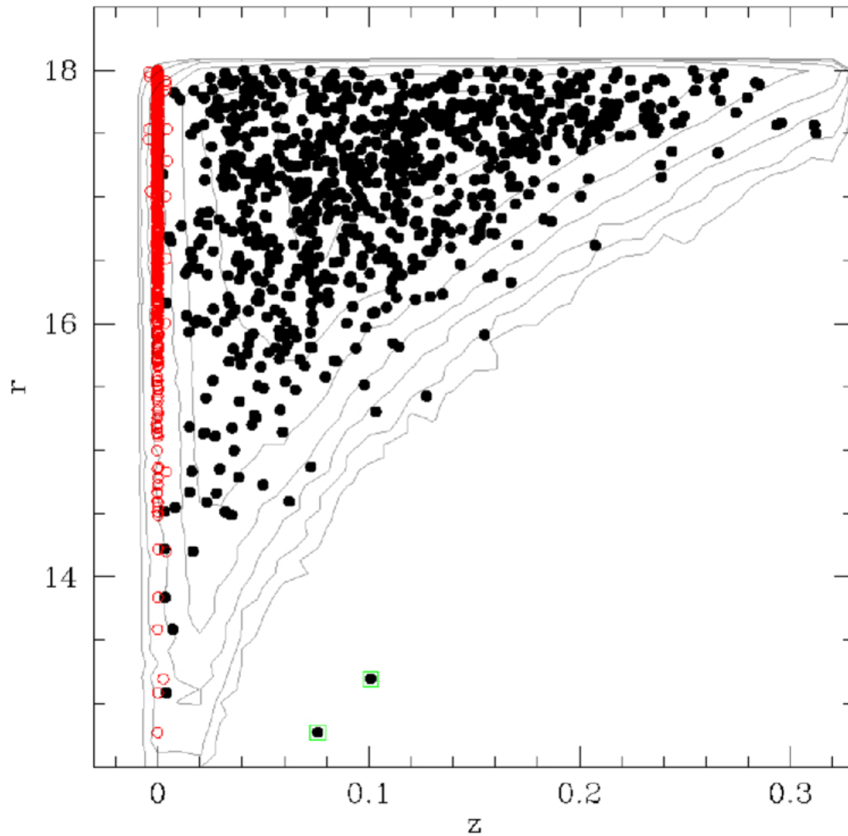
Figure 5. from Masafumi Yagi et al 2025 Astron. J. 170 doi:10.3847/1538-3881/ade543 https://dx.doi.org/10.3847/1538-3881/ade543 © 2025. The Author(s). Published by the American Astronomical Society.
