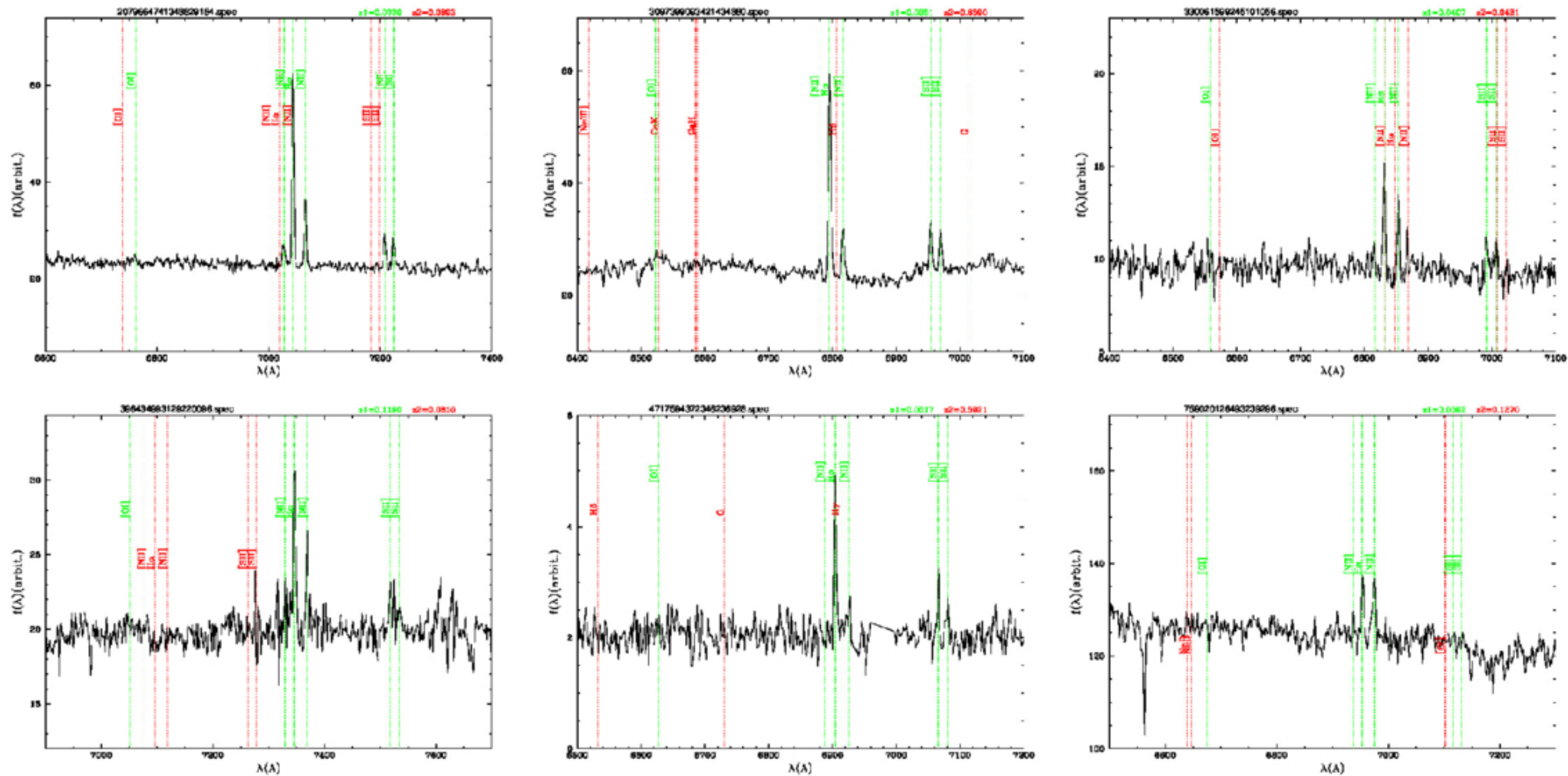
Figure 4. from Masafumi Yagi et al 2025 Astron. J. 170 doi:10.3847/1538-3881/ade543 https://dx.doi.org/10.3847/1538-3881/ade543 © 2025. The Author(s). Published by the American Astronomical Society.
