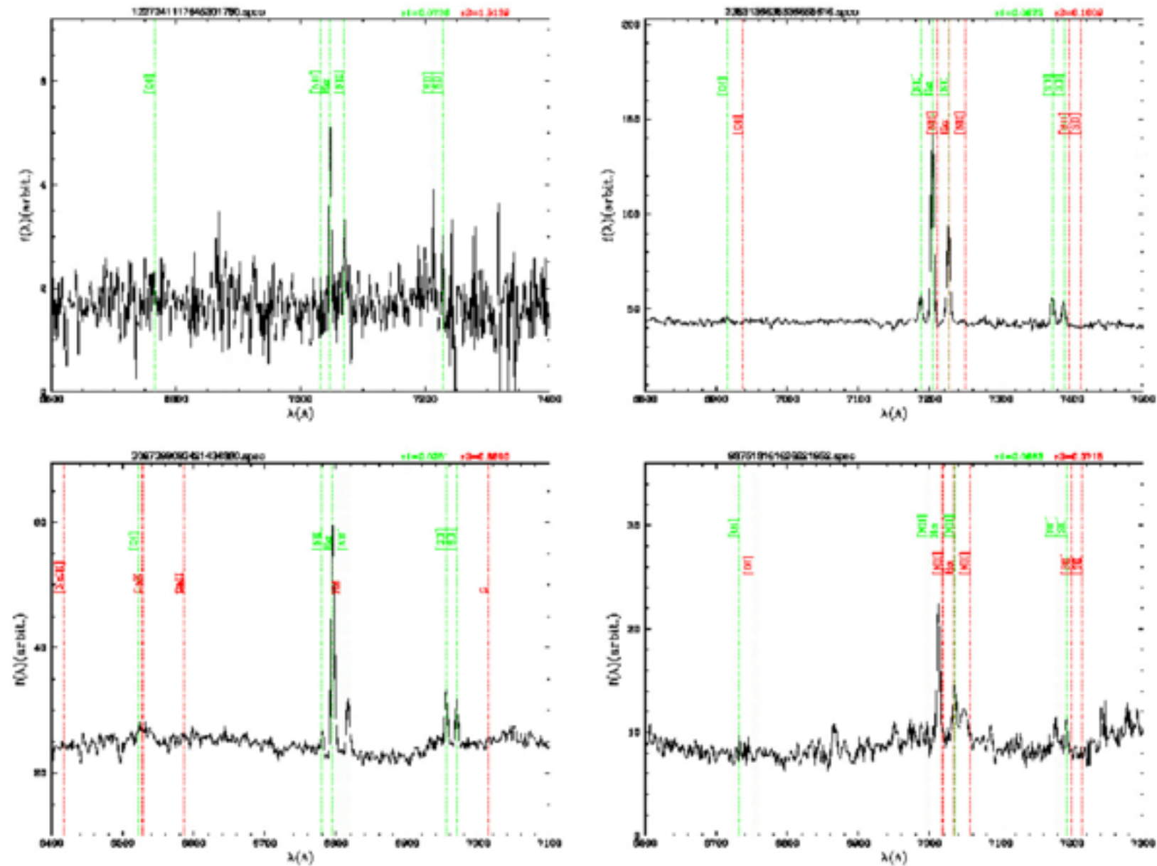
Figure 3. from Masafumi Yagi et al 2025 Astron. J. 170 doi:10.3847/1538-3881/ade543 https://dx.doi.org/10.3847/1538-3881/ade543 © 2025. The Author(s). Published by the American Astronomical Society.
