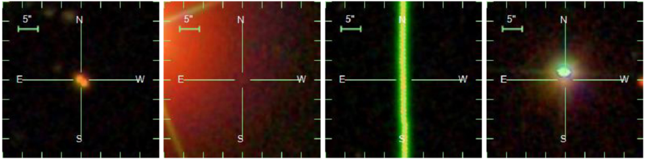
Figure 1. from Masafumi Yagi et al 2025 Astron. J. 170 doi:10.3847/1538-3881/ade543 https://dx.doi.org/10.3847/1538-3881/ade543 © 2025. The Author(s). Published by the American Astronomical Society.
