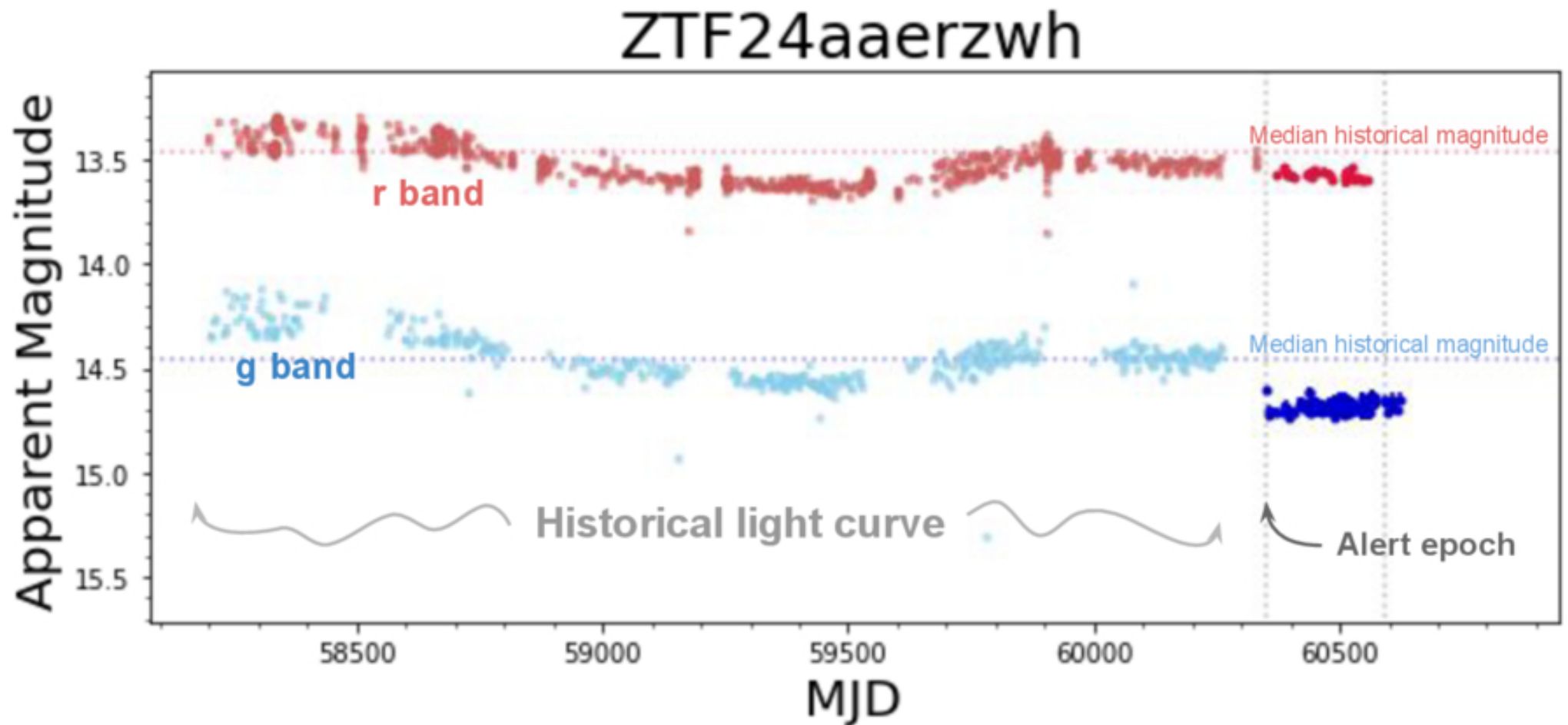
Figure 4. from Eleanor M. Galloway et al 2025 Astron. J. 170 doi:10.3847/1538-3881/ade4bb https://dx.doi.org/10.3847/1538-3881/ade4bb © 2025. The Author(s). Published by the American Astronomical Society.
