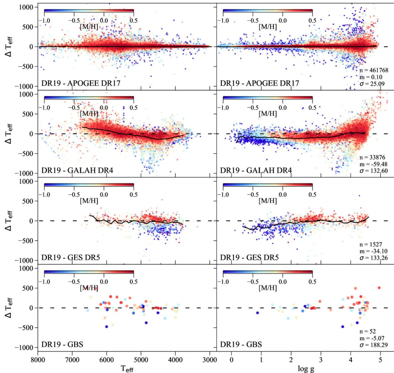
Figure 4. from Szabolcs Mészáros et al 2025 Astron. J. 170 doi:10.3847/1538-3881/ade4b9 https://dx.doi.org/10.3847/1538-3881/ade4b9 © 2025. The Author(s). Published by the American Astronomical Society.
