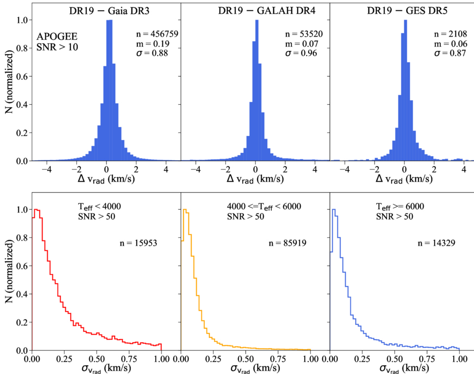
Figure 2. from Szabolcs Mészáros et al 2025 Astron. J. 170 doi:10.3847/1538-3881/ade4b9 https://dx.doi.org/10.3847/1538-3881/ade4b9 © 2025. The Author(s). Published by the American Astronomical Society.
